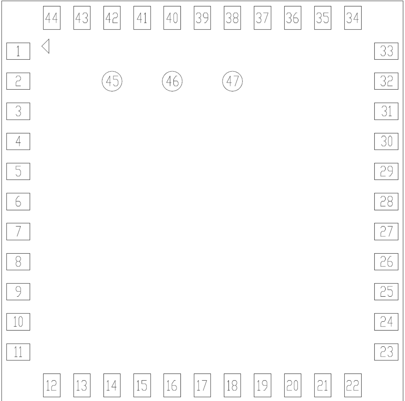
•Top View of PCB Layout Foot Print
