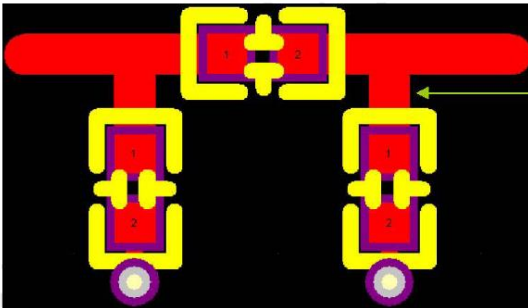
Incorrect layout for antenna matching
