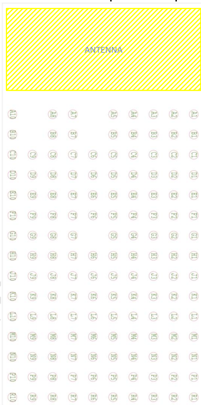
AW-CU427 Top View Pin Map
