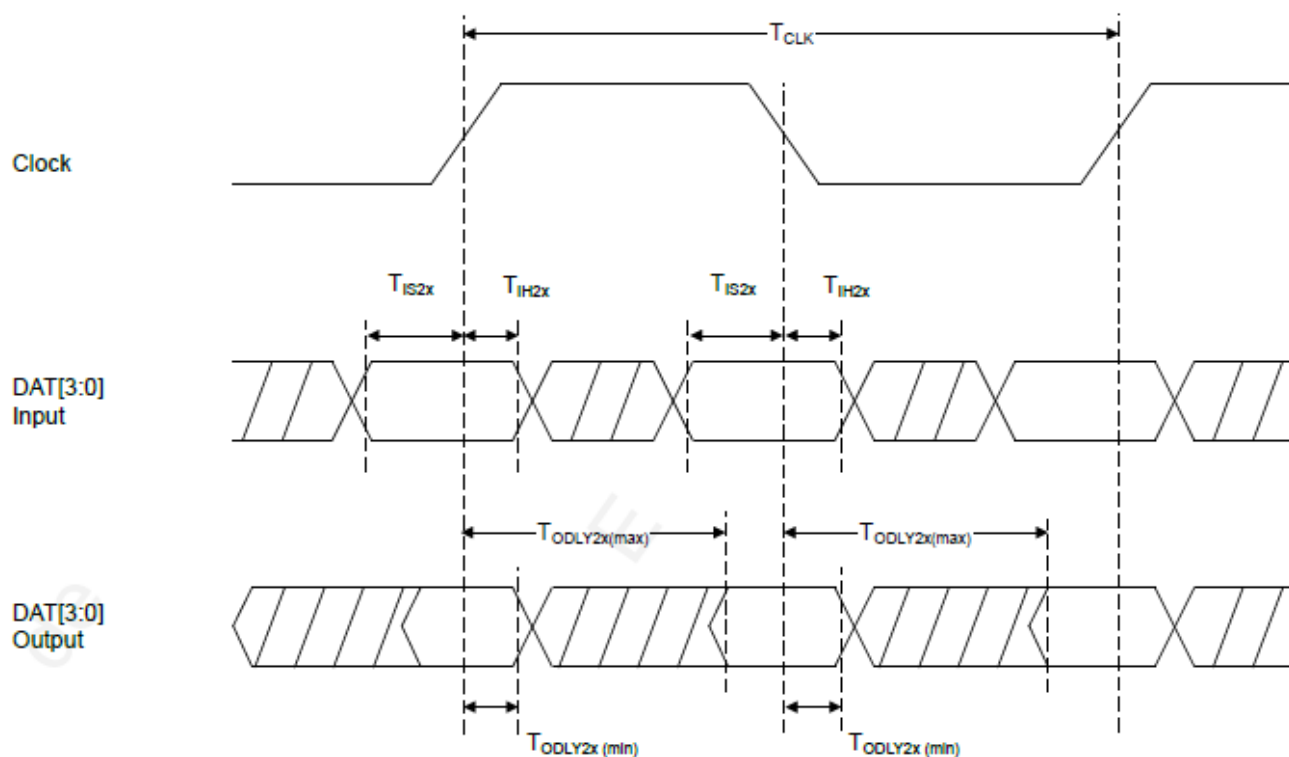
SDIO DAT[3:0] timing diagram—DDR50 mode(50 MHz)
