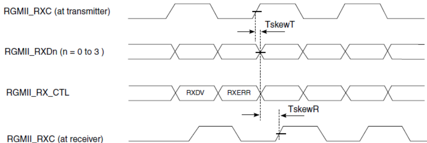
Figure 7. RGMII receive signal timing diagram original
