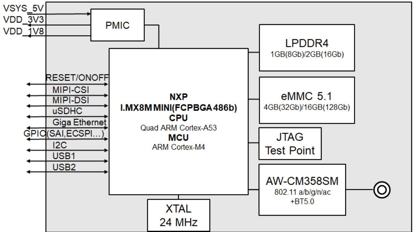
AW-PU510 Block Diagram
