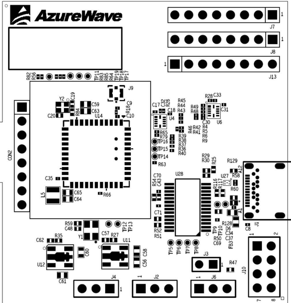
Top View
