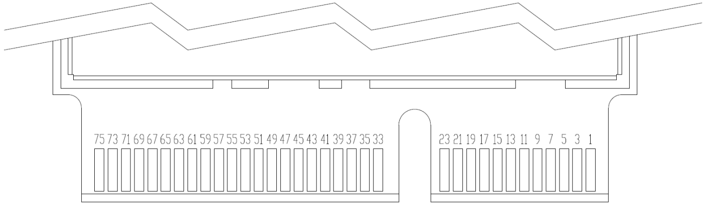
AW-CB511NF-BPF Pin Map (Top View)
