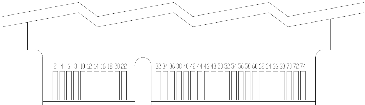
AW-CB511NF-BPF Pin Map (Bottom View)
