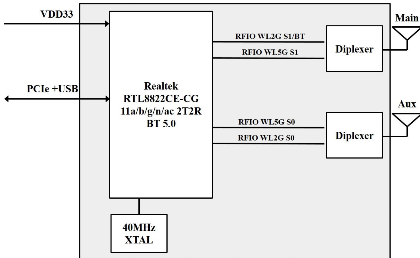
AW-CB375NF BLOCK DIAGRAM
