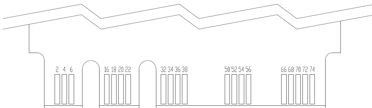
AW-CB375NF Pin Map (Bottom View)
