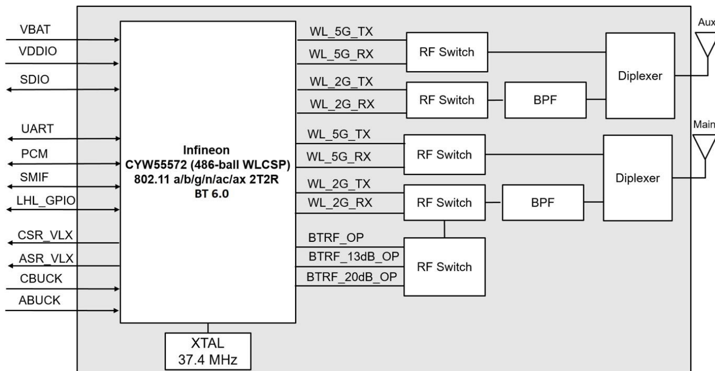
AW-XH327-SUR Block Diagram
