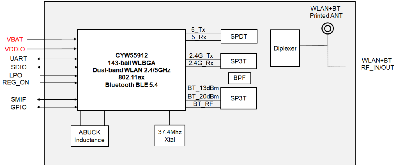
AW-CU642 Block Diagram
